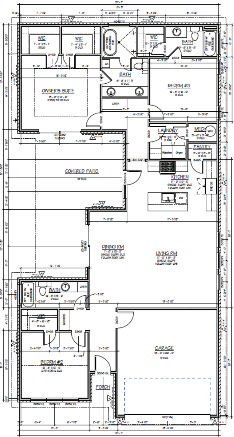
2 FLOOR PLAN 1/4" = 1'-0"
